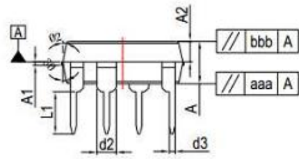
Right View
