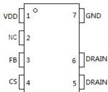
PL3325CS (SOP7)/ PL3325CD/H(DIP7)
